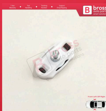
BWR5613 Front Window Regulator Sliding Pivot Guide Jaw Clips for Vauxhall Opel Astra H 2004-2014 Vectra C Z02 2002-2009 4/5 Door
