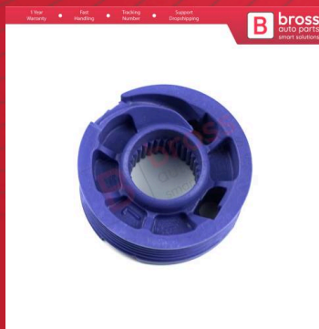
BWR131 Window Regulator Repair Cable Roll Gear Reel Wheel Pulley Front-Rear Left Door for Polo Toledo A3 C5 Phaeton 8V48394...
