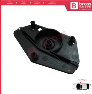
BWR5160 Window Regulator Repair Motor Cover Front Right for Citroen C4 Picasso MK1 UD Grand UA 2006-2013 MPV 9222CT
