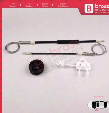
BWR797 Power Window Regulator Repair Set Front Left for Fiat Albea Siena Palio MK1 171 172 178 1996-2016 4/5 Door 46786201
