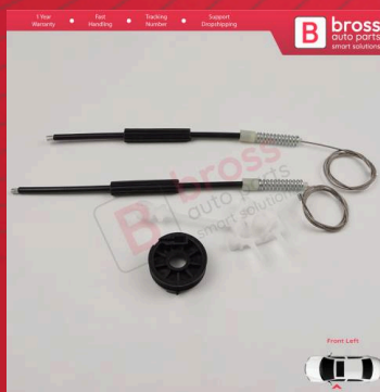
BWR264 Window Regulator Repair Kit Front Left Door for Fiat Doblo MK1 MPV Van 119 223 2001-2010 51718404
