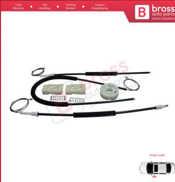
BWR818+BWR5157 Power Window Regulator Repair Set Front Left for Citroen C4 Picasso MK1 UD Grand UA 2006-2013 MPV 9221CV
