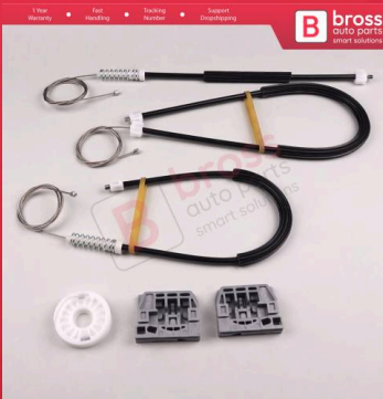
BWR275 Window Regulator Repair Kit Front Right Door for VW Caddy MK3 2K 2C 2004-2015 Van MPV 2K1837730
