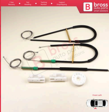
BWR644 Window Regulator Repair Kit Front Left Door for Peugeot 307 4/5 Door 2000-2008
