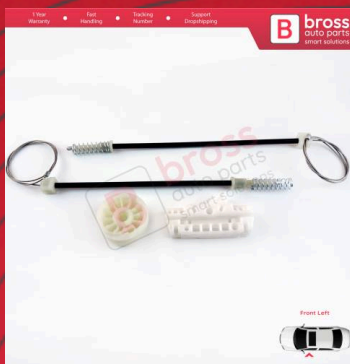
BWR5377 Power Window Regulator Repair Set Front Left for Opel Corsa D S07 2006-2014 5-Door 13188490
