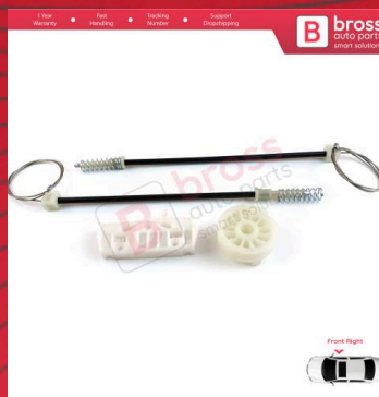
BWR5378 Power Window Regulator Repair Set Front Right for Opel Corsa D S07 2006-2014 5-Door 13188491
