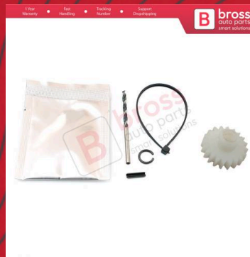
BGE578 Seat Height Adjuster Motor 5609510 Plastic Gear for Ford Mondeo Galaxy S Max Jaguar
