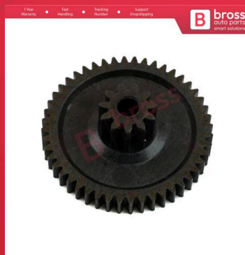
BGE658 Air Throttle Valve 03F133062B Gear 48/11 Teeth for Audi VW Seat Skoda 1.2 1.4 TSI Motor
