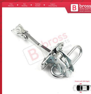
BDP1282 Front Door Hinge Stop Check Strap Limiter for Fiat Idea Lancia Musa 350 2004-2012 51795854
