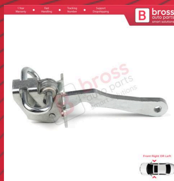
BDP693 Front Door Hinge Stop Check Strap Limiter 1328196080 for Fiat Ducato MK2 230 244 1994-2006
