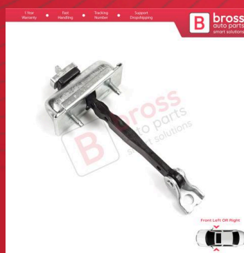
BDP1552 Front Door Stop Check Assy Limiter Strap for Vauxhall Opel Insignia B Z18 2017-On Buick Regal MK6 2018-2020 39089087
