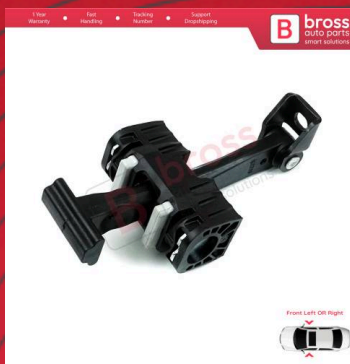
BDP1080 Front Door Hinge Brake Stop Check Strap Limiter 51217176809 for BMW 1 Series E87
