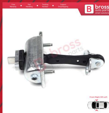
BDP733 Front Door Hinge Stop Check Strap Limiter 6C1AV23500AC for Ford Transit MK7 2006-2014 Tourneo
