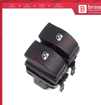
BDP849 Window Control Switch 10 Pin for Renault Trafic MK2 Espace 4 Scenic 2 Megane 2 Vauxhall Opel Movano A Vivaro 1...
