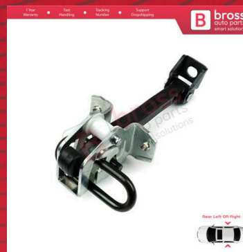
BDP1082 Rear Door Hinge Brake Stop Check Strap Limiter 51228160963 for BMW 3 E46 Saloon Estate
