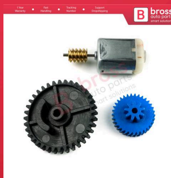
BGE662+BDP153 Driver Door Lock Actuator Motor Repair Gear Motor 9T1Z6121813B for Ford Transit Connect MK1 2002-2013
