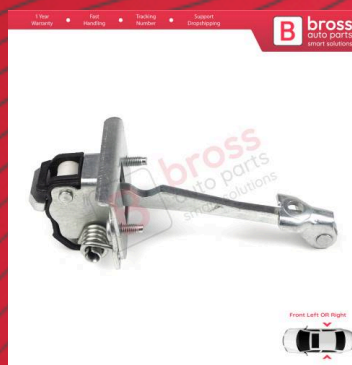
BDP785 Rear Door Hinge Stop Check Strap Limiter 9181.N3 for Peugeot 308 MK1 4/5 Door 2007-2013
