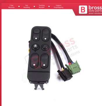
BDP730 Power Window Switch 1240600 for Opel Vectra A Cavalier
