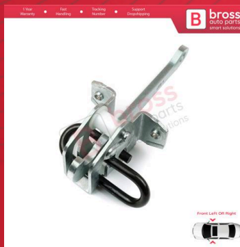
BDP1063 Front Door Hinge Brake Stop Check Strap Limiter 51218165005 for BMW 3 E36
