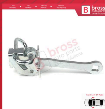
BDP727 Front Door Hinge Stop Check Strap Limiter 5160232 for Vauxhall Opel Omega B Catera
