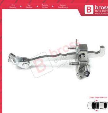
BDP711 Front Door Hinge Stop Check Strap Limiter 7700311823 for Renault Trafic MK2 Vivaro A PriMastar X83
