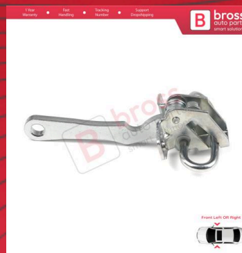
BDP779 Front Door Hinge Stop Check Strap Limiter 918179 for Citroen Jumper MK1 230 244 1994-2006
