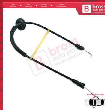
BDP71 Front Inner Door Lock Release Latch Bowden Cable for VW Golf MK5 1K1 1K5 Plus 5M1 521 Jetta MK3 1K2 4/5 Door...
