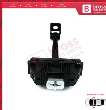
BDP1079 Front Door Hinge Brake Stop Check Strap Limiter 51218402502 for BMW X5 E53
