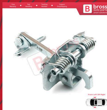
BDP937 Front Door Hinge Stop Check Strap Limiter 9181E6 for Citroen Xsara Picasso 1999-2012
