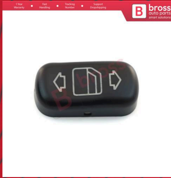
BDP111 1 Piece Rounded Edge Window Switch Button Cover for Mercedes E Class W210 S210 C Class W202 S202 2108208210
