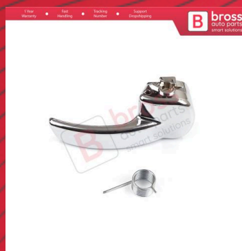
BDP915 Interior Front or Rear Right Door Chrome Handle 80670JD00E For Nissan Qashqai Dualis 2007-2013 J10 JJ10
