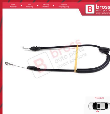
BDP67 Inner Door Release Latch Bowden Cable Front Left 53 cm For VW Caddy MK3 2K 2004-2015 Touran MK1 1T 2003-2015 2K0837113B
