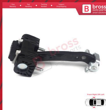
BDP695 Front Door Hinge Stop Check Strap Limiter 9181N9 for Fiat Ducato Peugeot Boxer Manager 250 290 2006-On
