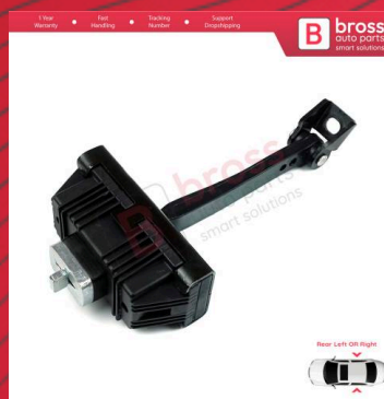
BDP1083 Rear Door Hinge Brake Stop Check Strap Limiter 41527176802 for BMW X3 E83 2003-2011
