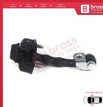
BDP692 Front Door Hinge Stop Check Strap Limiter 4694080 for Fiat Doblo 263 Citroen Nemo Peugeot Bipper Opel...
