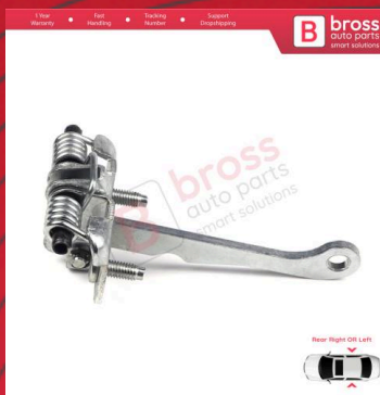
BDP938 Rear Door Hinge Stop Check Strap Limiter 9181H4 for Peugeot 106 1991-2004 Citroen Saxo 1996-2004
