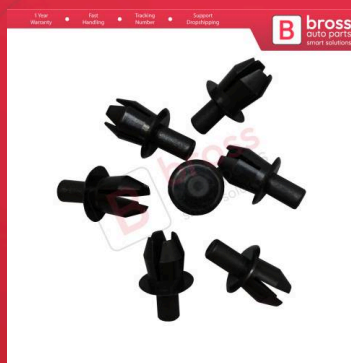
BCF5060 10 Pieces Push Type Retainer Black for Mercedes 1239900292 VW Audi N0385501 Seat N0385501 Ford 7200671
