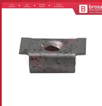
BCF2432 10 Pieces Spring Nut for Mercedes Benz 12.8x18.5x11.3mm
